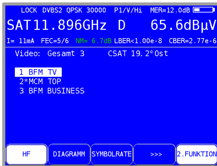
Abbildung 7-7 SAT DVB-S/S2-Parameter
