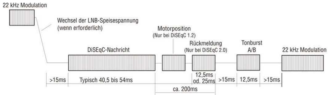
Abbildung 7-12 DiSEqC 1.0 Sequenz
