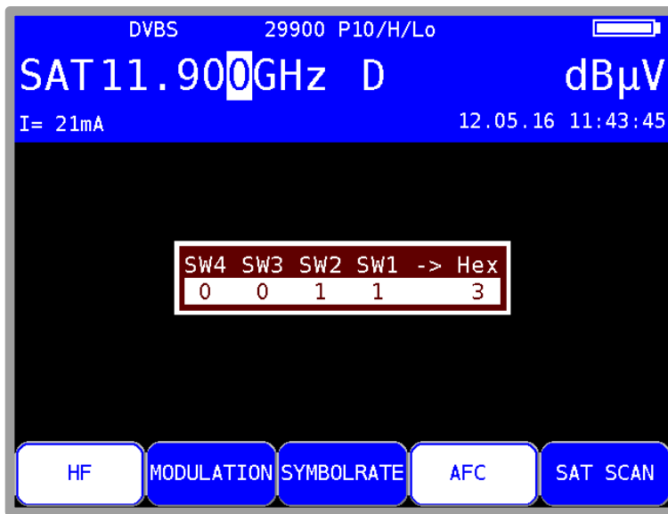
Abbildung 7-12 DiSEqC 1.1 Uncommitted Switches
